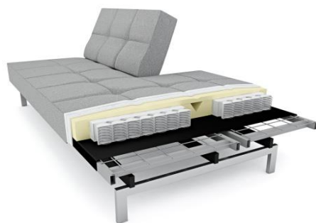
Cross-section-view
